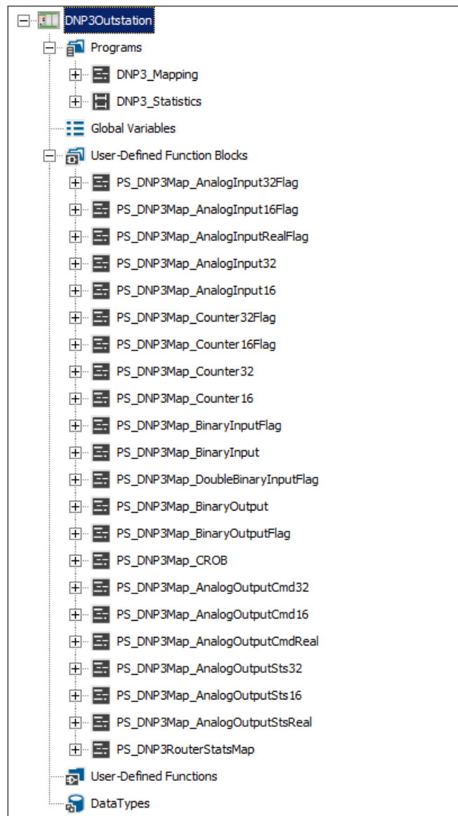
Figure 5 - Project Explorer
