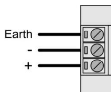
Figure 2.5 - Power connector
