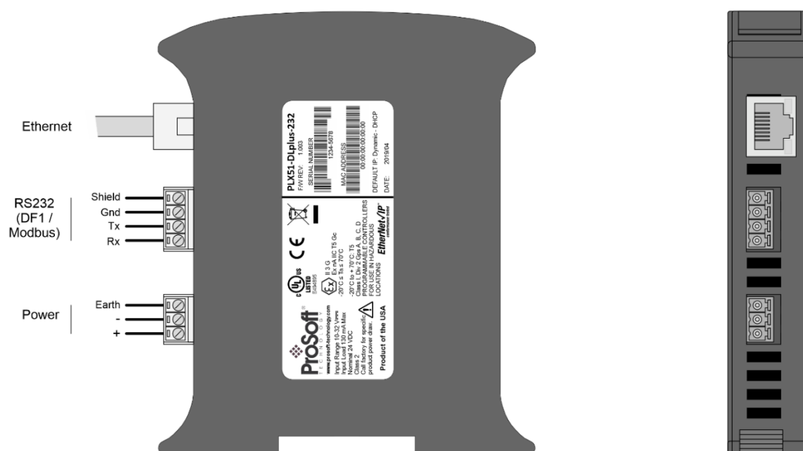
Figure 2.1 –Side and bottom view
