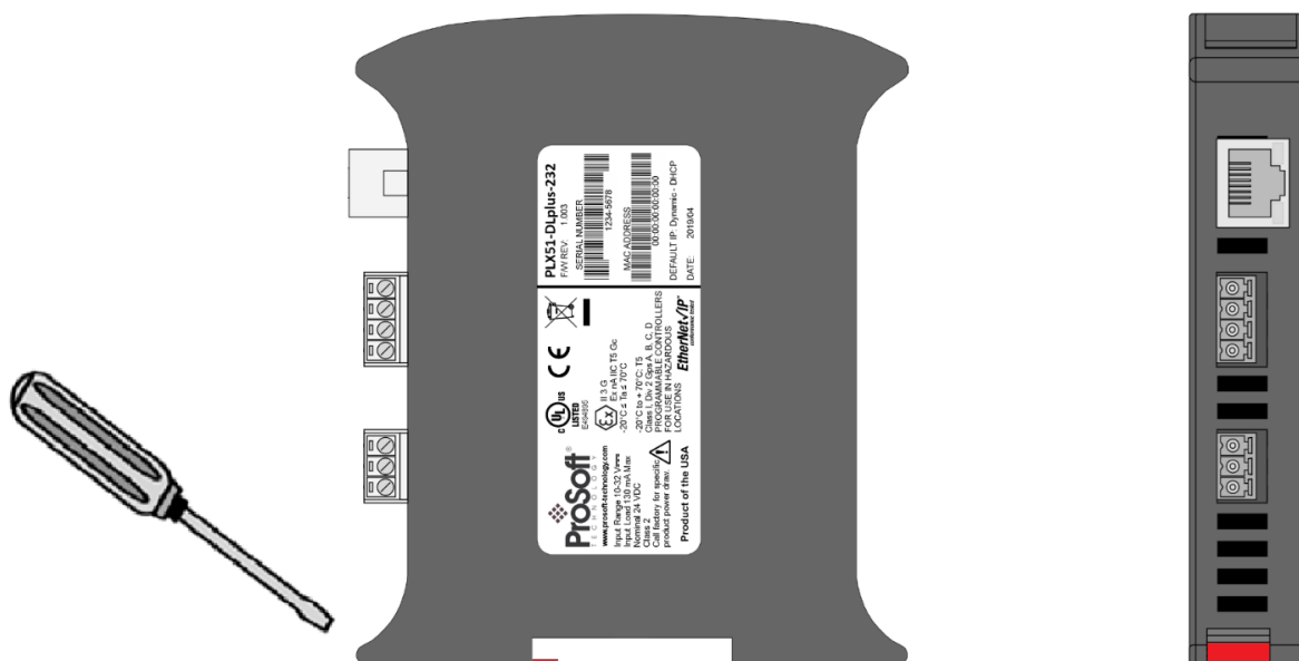
Figure 2.4 - DIN rail mounting
