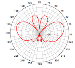
RMM 925 MHz – Azimuth Plot
