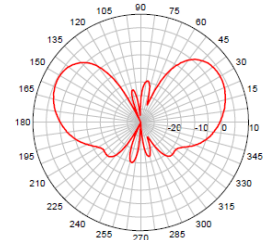
RMM 1900 MHz – Elevation Plot
