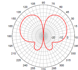
RMM 925 MHz – Elevation Plot
